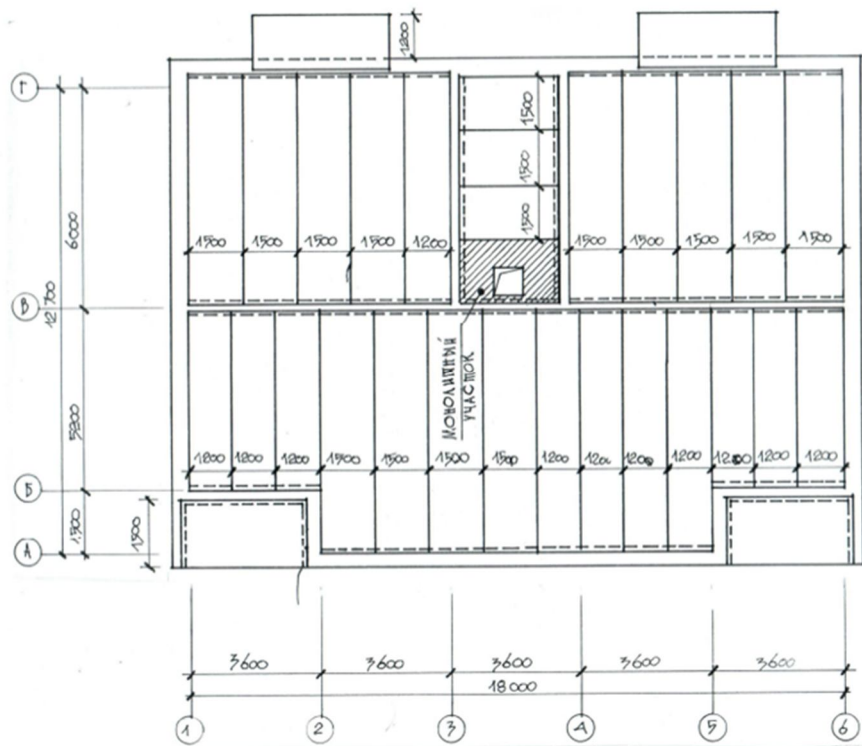
Figure A.6 – Plan of floor slabs (Scale 1:100)
