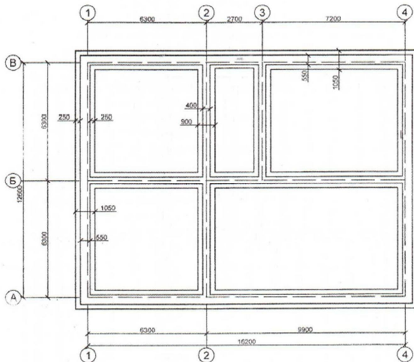
Figure A.2 – Plan of stripe foundation (Scale 1:100)
