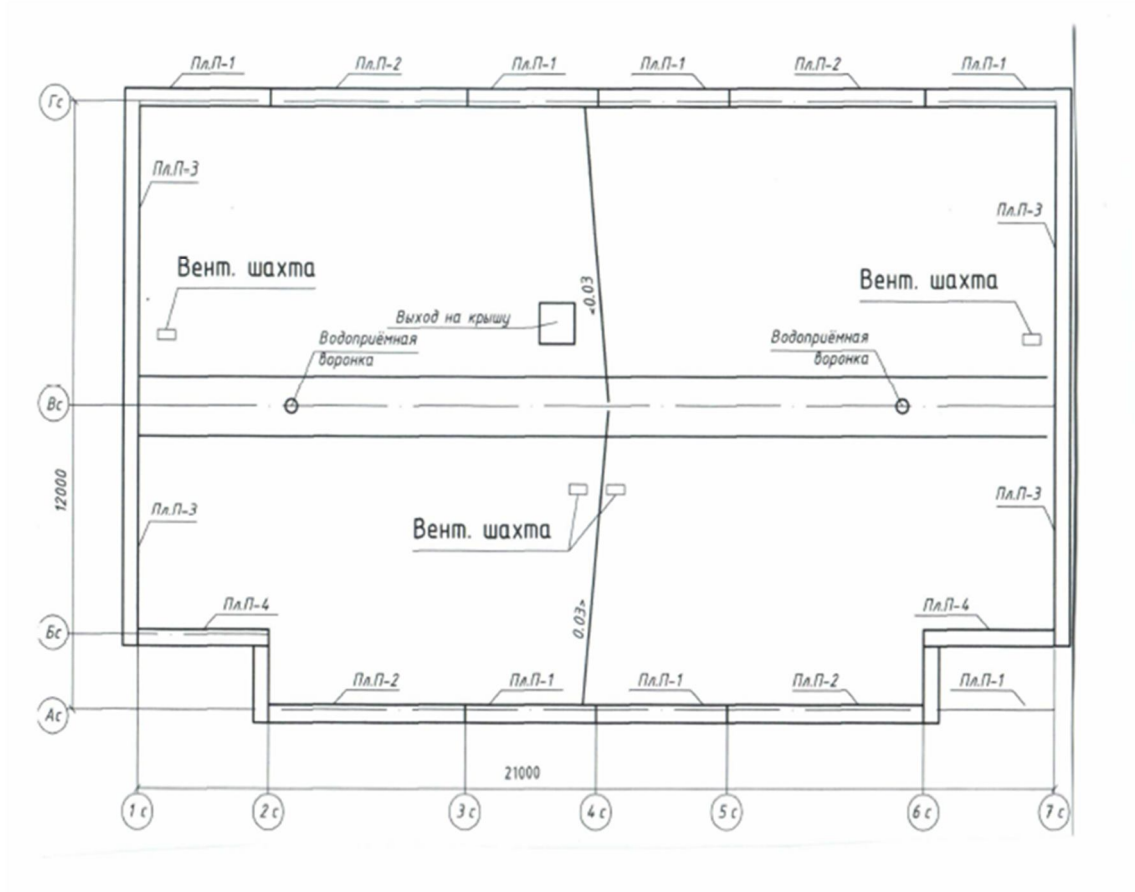
Figure A.7 – Plan of roof (Scale 1:100)
