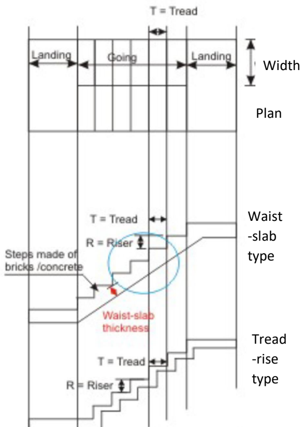
Figure 3 – Typical flight
