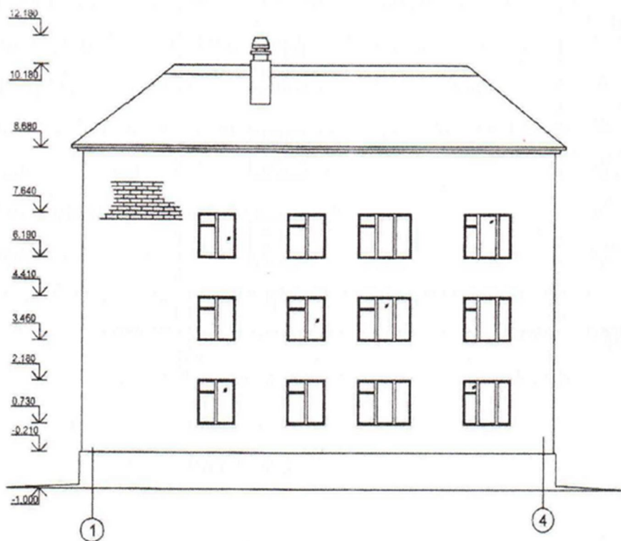
Figure A.4 – Main Elevation (Scale 1:100)
