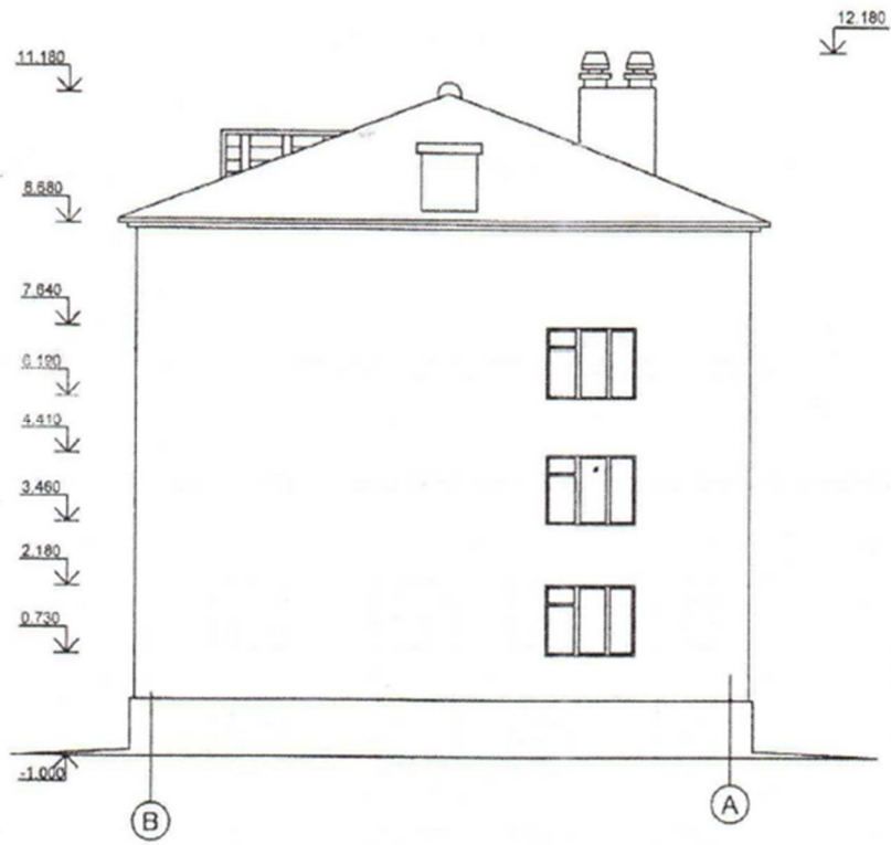
Figure A.5 – Side Elevation (Scale 1:100)
