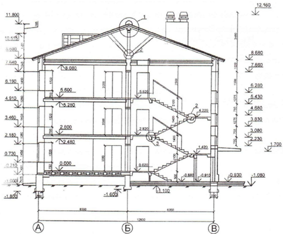
Figure A.3 – Vertical cross-section A-A (Scale 1:100)
