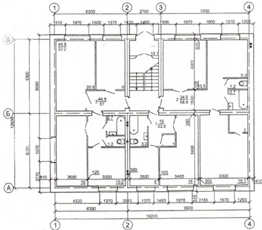
Figure A.1 – Plan of the first floor (Scale 1:100)
